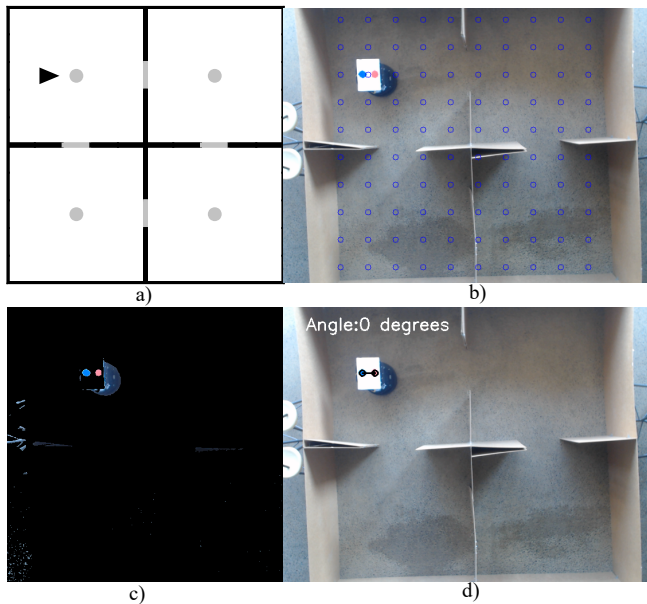
Fig. 1. Visualisation and real world correspondence of the low fidelity simulation of the real four-rooms domain. a) The agent in the abstract skill-level simulator. b) Centres of each grid-state displayed on top of the overhead camera feed. c) Segmentation mask for robot and colour tags identification in the overhead camera feed. d) Localisation of the robot with position and angle in the real world four rooms domain.
