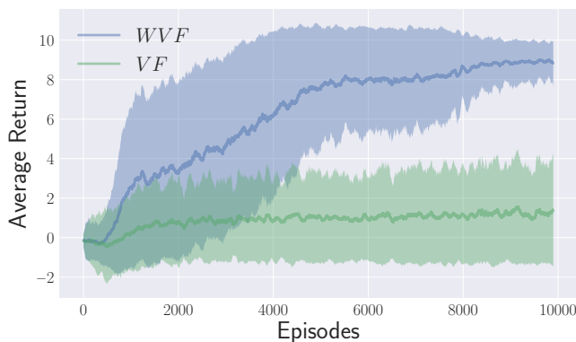
Fig. 5. Average returns per episode obtained when learning WVFs and regular VFs in the four-rooms simulation. The shaded regions represent 1 standard error over the returns obtained when training the following 10 tasks: Navigate to the "bottom-left room", "bottom-right room", "top-right room", "top-left room", "front of left door", "front of top door", "front of right door" and "front of bottom door".
